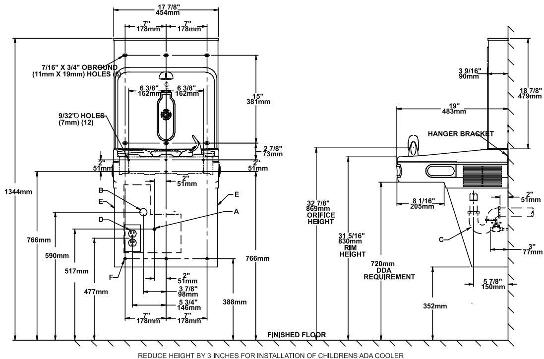
REDUCE HEIGHT BY 3 INCHES FOR INSTALLATION OF CHILDRENS ADA COOLER
